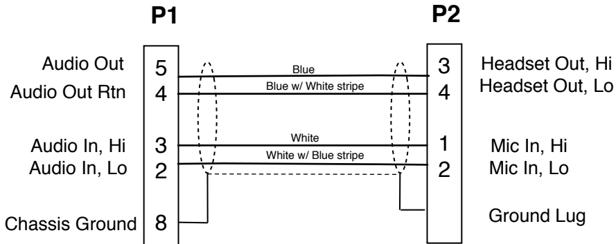
Wiring Diagram Pins Not Shown Are Unused
